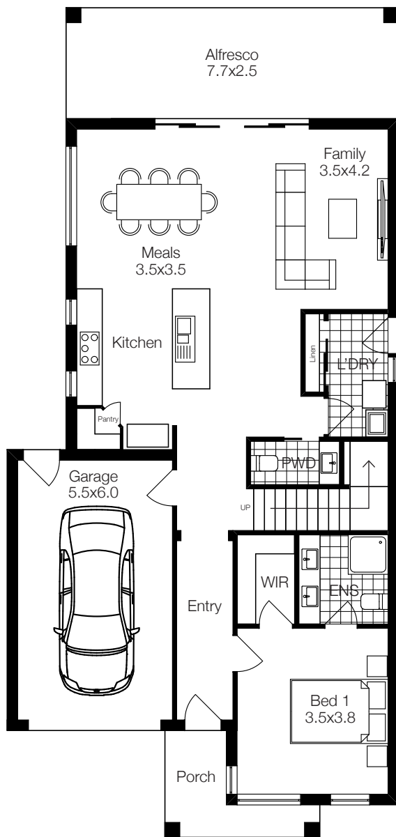
GROUND FLOOR
