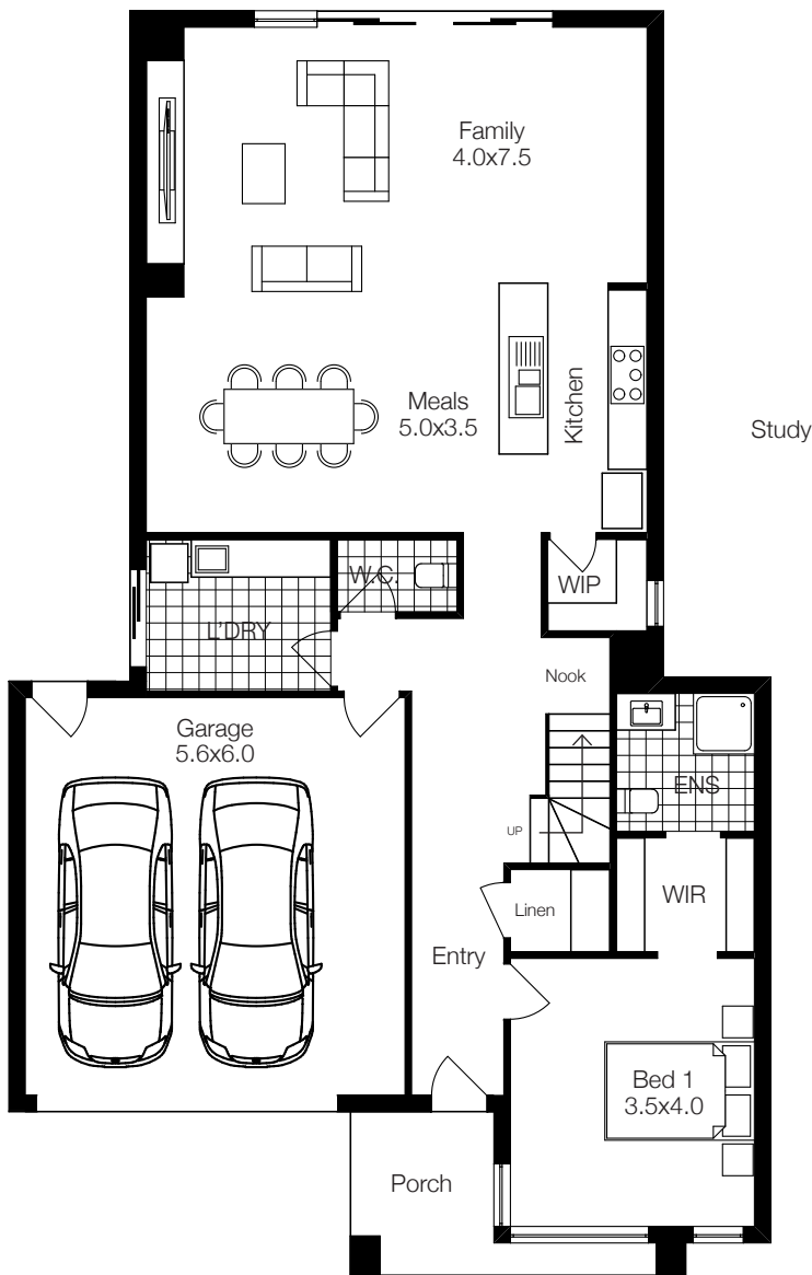
GROUND FLOOR
